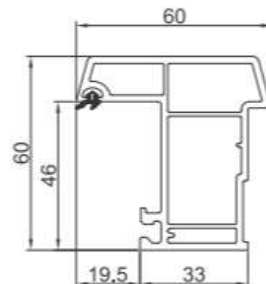
GB31mm FP-021-1 0.24 Kg/m Length (m) 5.9 30 Pcs (Per Pack)
