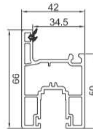
Window Sash FP-033 0.91Kg/m Length (m) 5.9 10 Pcs (Per Pack)
