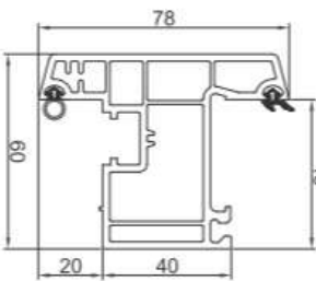
Outward Window Sash FP-015 1.15 Kg/m Length (m) 5.9 6 Pcs (Per Pack)
