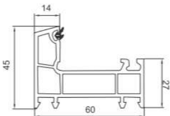
Frame FP-011 0.850 Kg/m Length (m) 5.9 8 Pcs (Per Pack)
