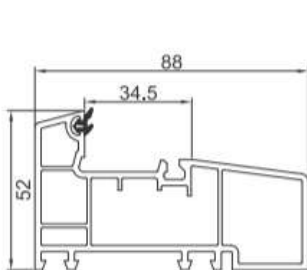
Fixed Frame FP-203-1 1.09Kg/m Length (m) 5.9 6 Pcs (Per Pack)
